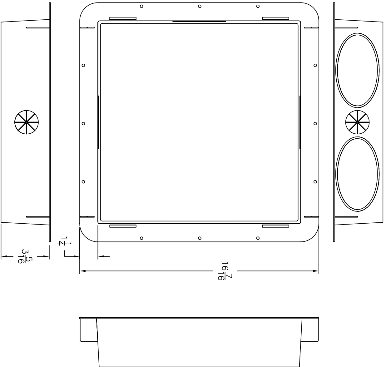
4" DBX1000 BOX DIMENSION VIEW
